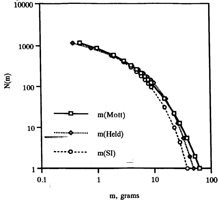
Figure 1. Comparison of Mott, Held, and Strømsøe and Ingebrigtsen (SI) equations for fragmentation, normalized to a common basis.
