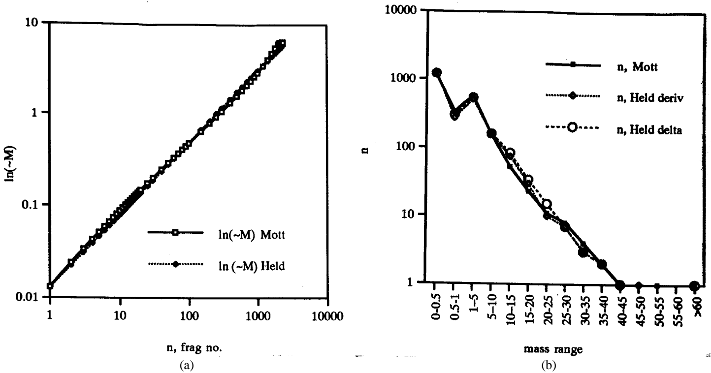
Figure 2. Comparison of Mott and Held formulations for (a) \ln(\sim M) = \ln[M/(M-M(n))] , and (b) number of fragments in individual mass ranges.
