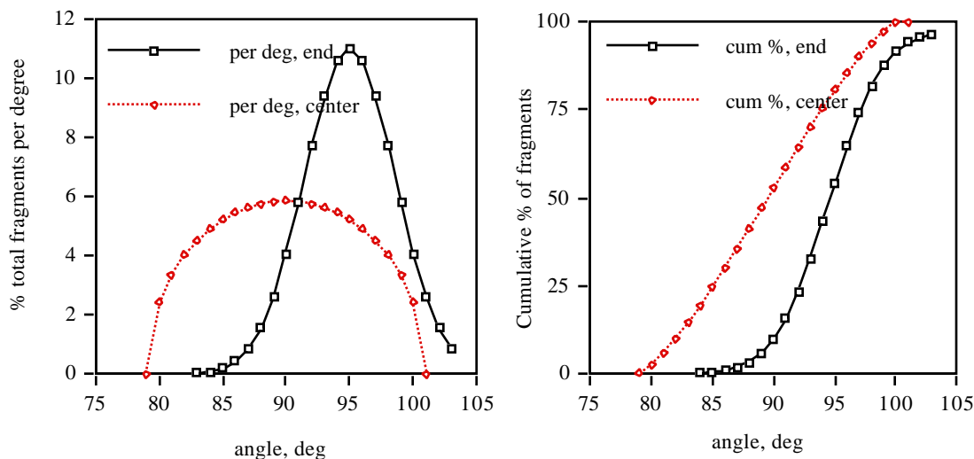
Figure 3a. Azimuthal differential percentage fragment spatial distribution, per degree for end- and center-initiated cylindrical warheads. Figure 3b. Azimuthal cumulative percentage fragment spatial distribution for end- and center-initiated cylindrical warheads.
